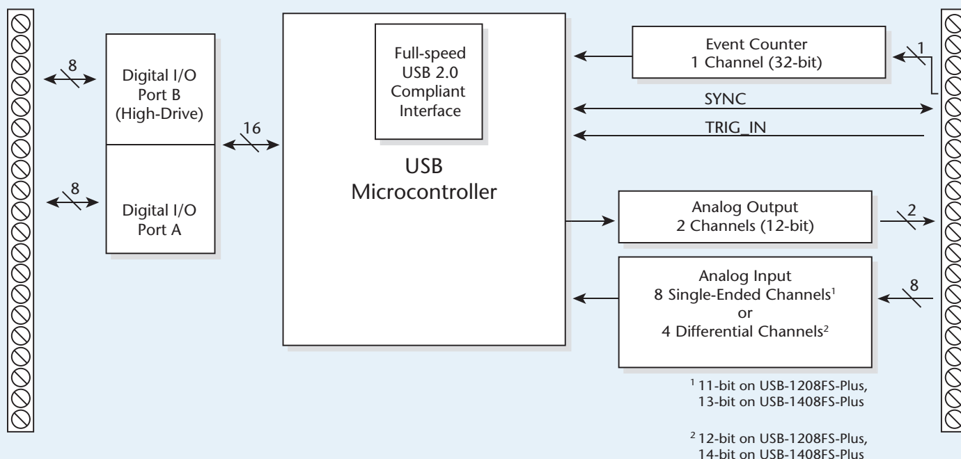
USB-1208FS-Plus and USB-1408FS-Plus Block Diagram
